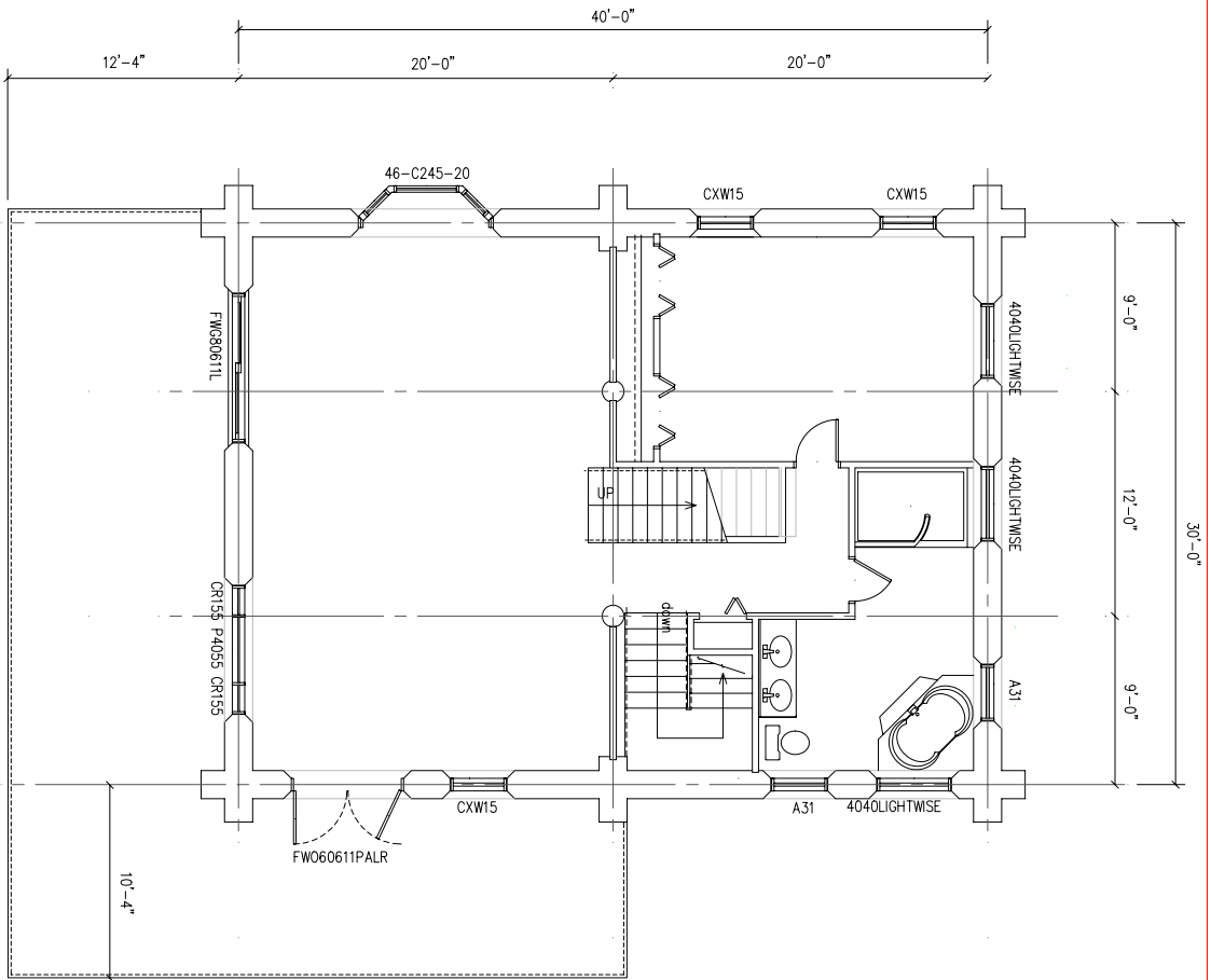
MAIN FLOOR/SECOND FLOOR FRAMING PLAN 1/8" = 1'-0"
