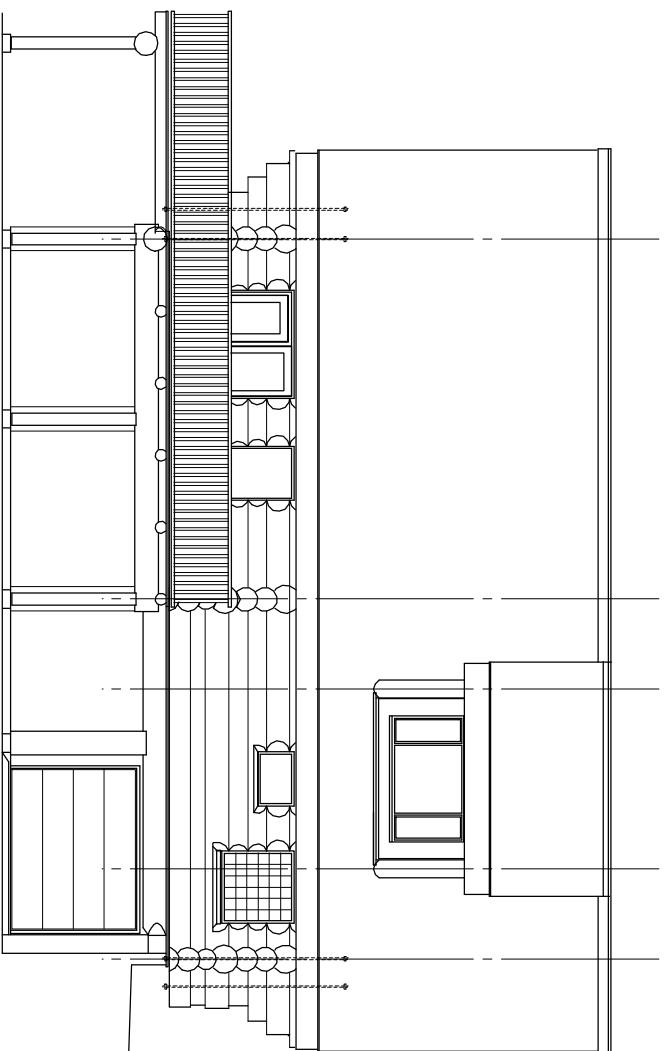
EAST ELEVATION 3/16" = 1'-0"
